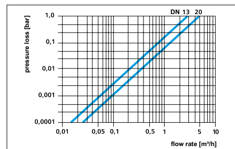
Head loss curves
